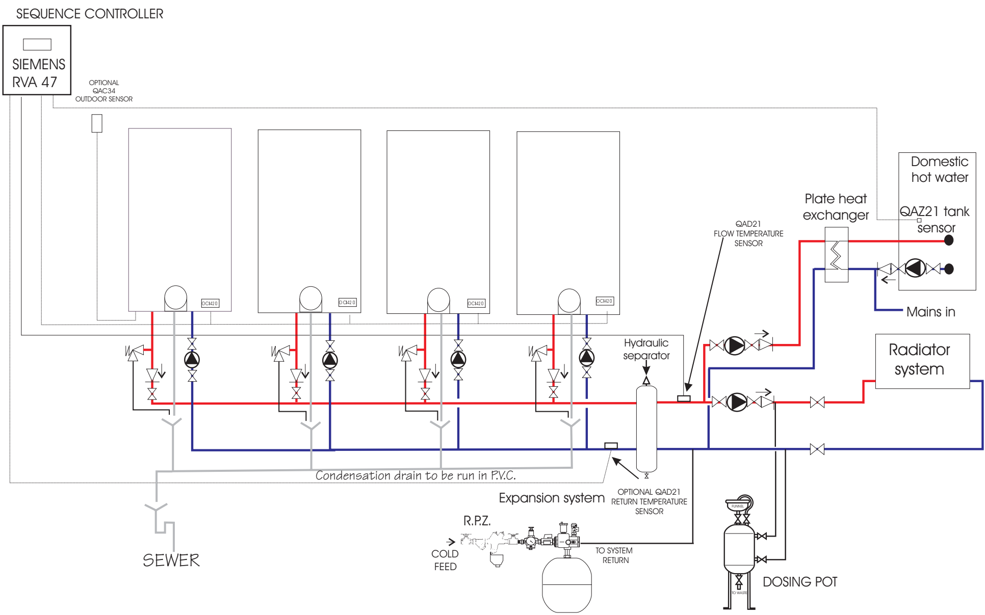
EXAMPLE OF 2-12 POWER HT FLOOR STANDING CONDENSING BOILERS IN CASCADE Heating and domestic hot water DRAWN: 17/11/08 BY: IVAN KARLAULA
